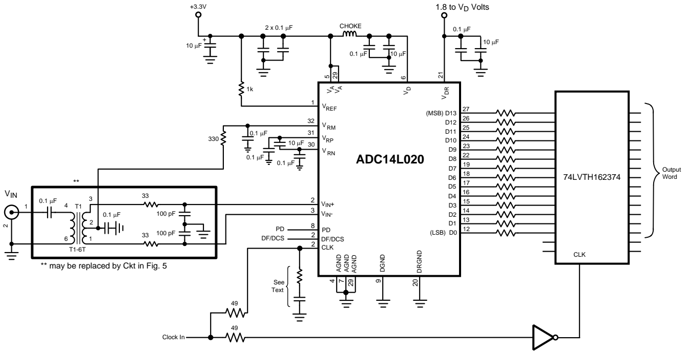
Figure 5. Application Circuit using Transformer Drive Circuit
