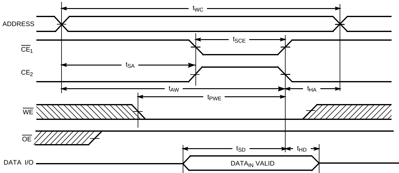
Write Cycle No. 2 ( \overline{CE_1} or CE_2 Controlled) [8, 12, 14]
