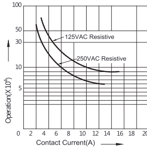
Life Curves
