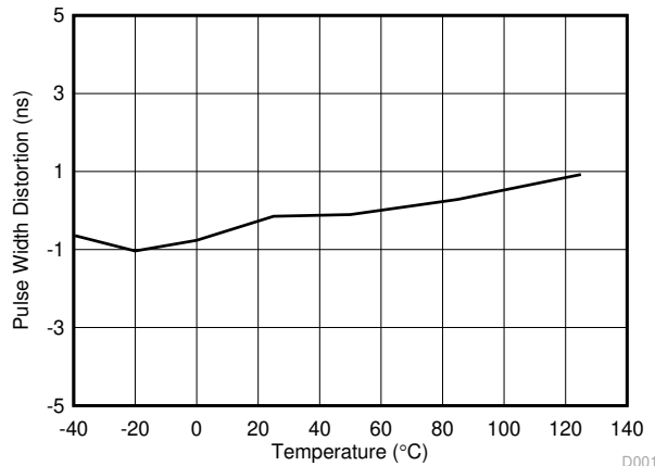
图 6-14. Pulse Width Distortion vs. Temperature
