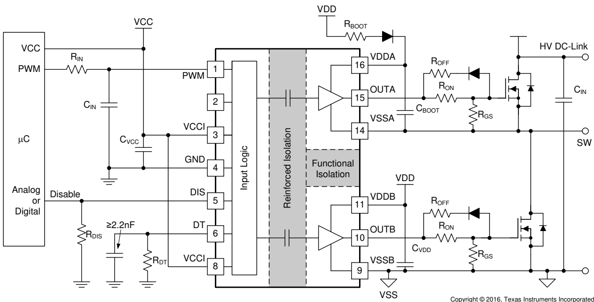
图 9-1. Typical Application
