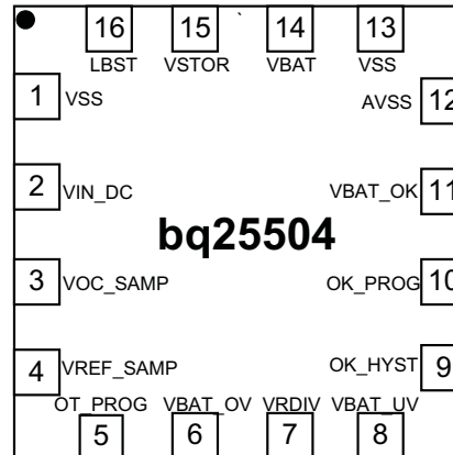
RGT Package 16 Pins Top View
