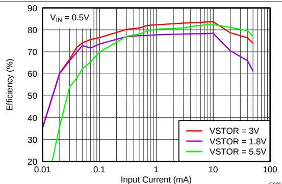
Figure 4. Efficiency vs Input Current
