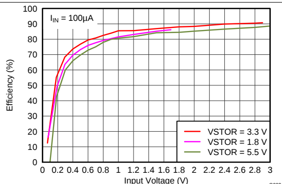
Figure 2. Efficiency vs Input Voltage
