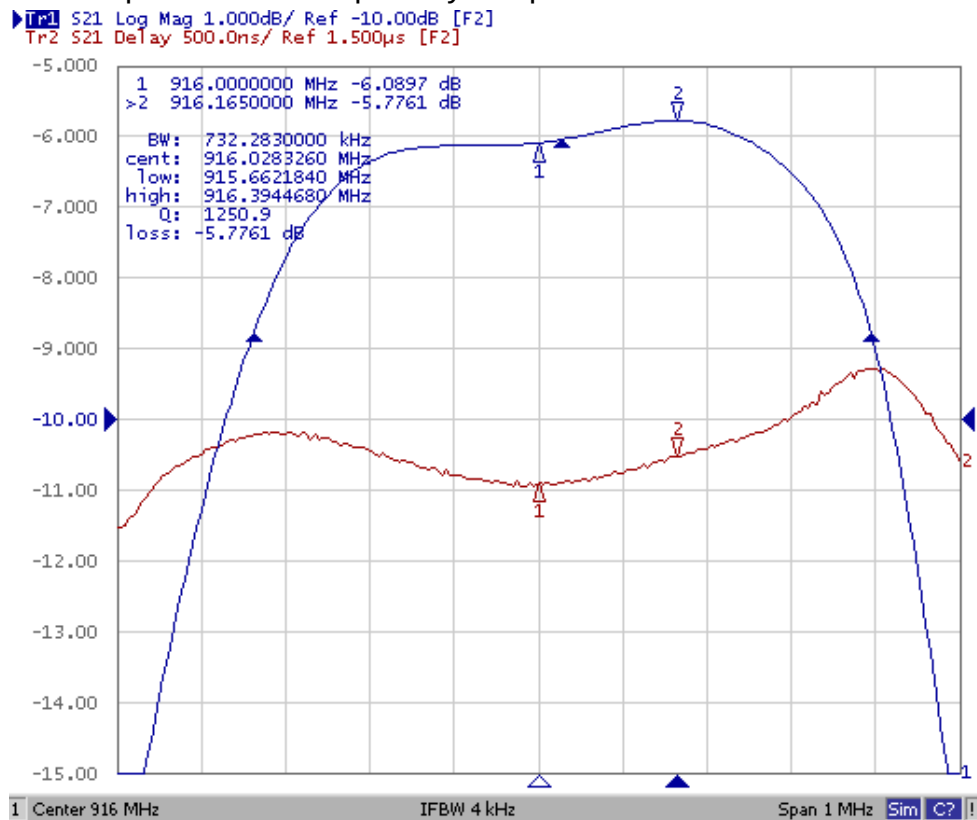
Fig2. Horizontal: 0.1MHz/Div Vertical: 1dB/Div
