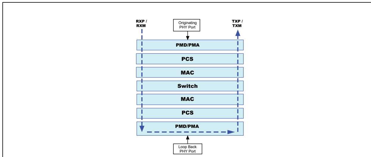
FIGURE 3-13: FAR-END LOOPBACK PATH
