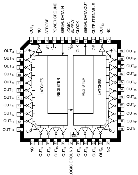
UCN5833EP
