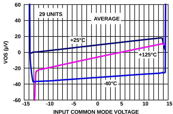
FIGURE 8. INPUT OFFSET VOLTAGE vs INPUT COMMON MODE VOLTAGE, V_S = \pm 15V
