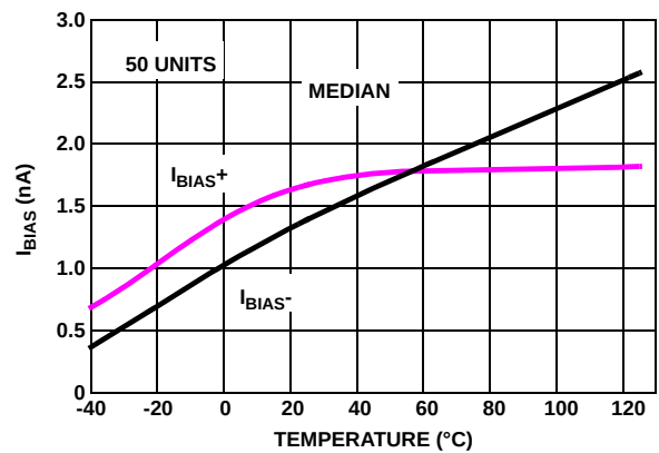
FIGURE 6. I_B vs TEMPERATURE, V_S = \pm 5V
