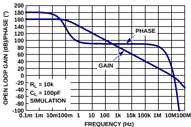
FIGURE 12. OPEN-LOOP GAIN, PHASE vs FREQUENCY, R_L = 10k\Omega , C_L = 100pF
