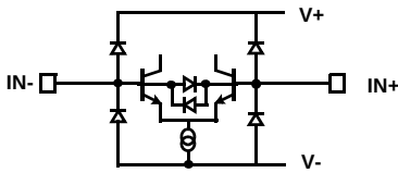
CIRCUIT 1
