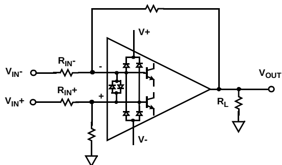
FIGURE 27. INPUT ESD DIODE CURRENT LIMITING - DIFFERENTIAL INPUT
