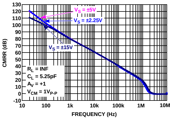
FIGURE 3. CMRR vs FREQUENCY, V_S = \pm 2.25 , \pm 5V , \pm 15V
