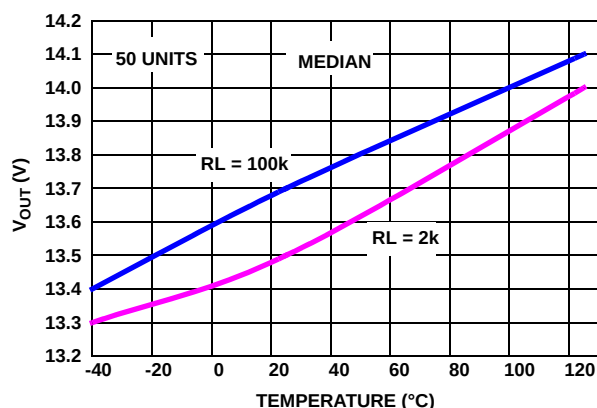
FIGURE 9. V_{OH} vs TEMPERATURE, V_S = \pm 15V
