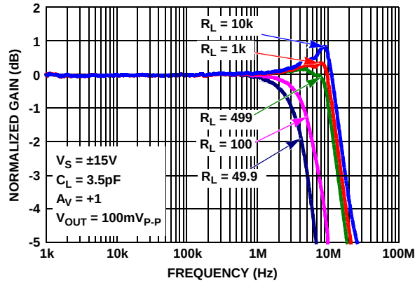
FIGURE 15. GAIN vs FREQUENCY vs R_L
