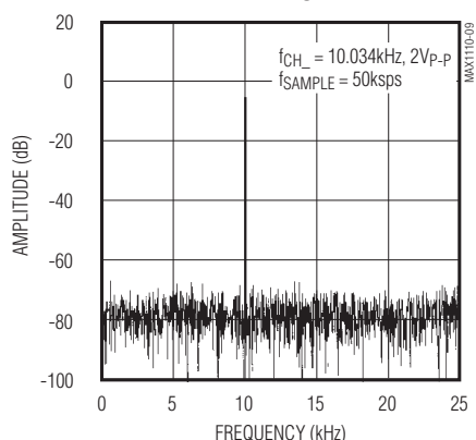
FFT PLOT
