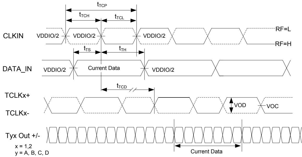
Figure 4. LVCMOS Input AC Timing Diagrams
