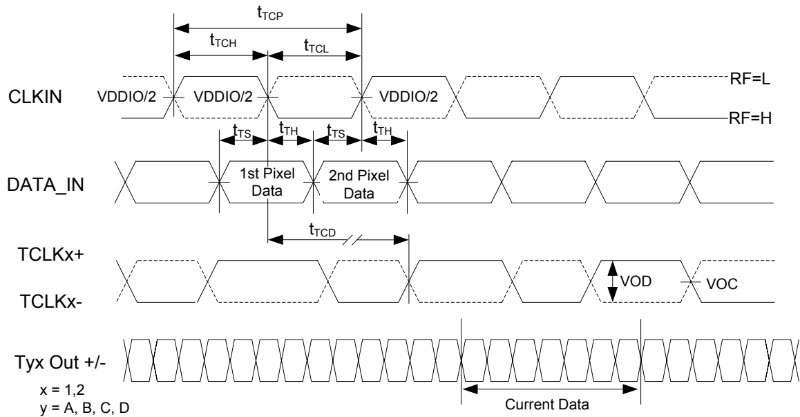
Figure 5. LVCMOS Input AC Timing Diagrams (DDRN=L)
