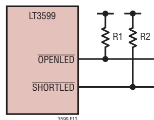
Figure 12. OPENLED and SHORTLED Connection
