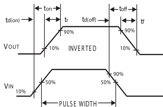
FIG.12 Switching Waveforms
