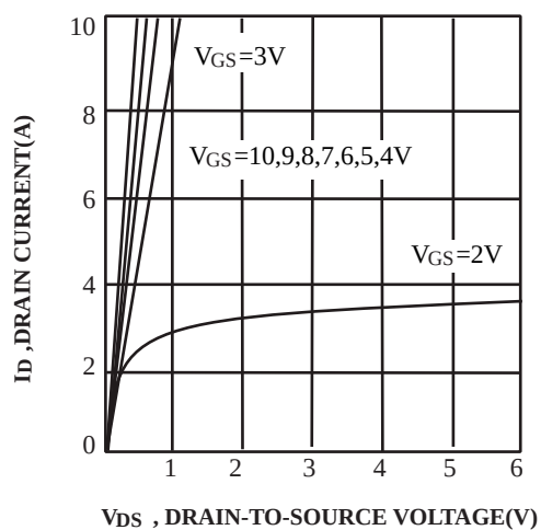
FIG.1. Output Characteristics
