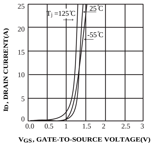
FIG.2 Transfer Characteristics
