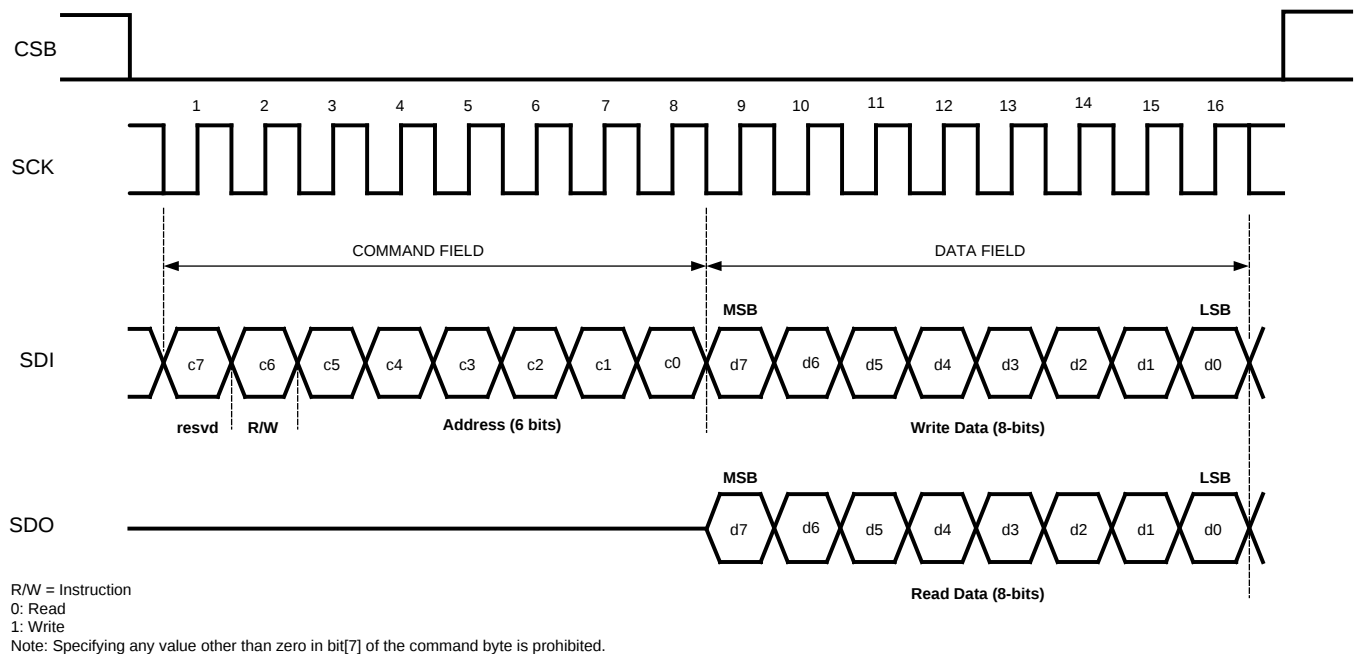
Figure 40. SPI Protocol
