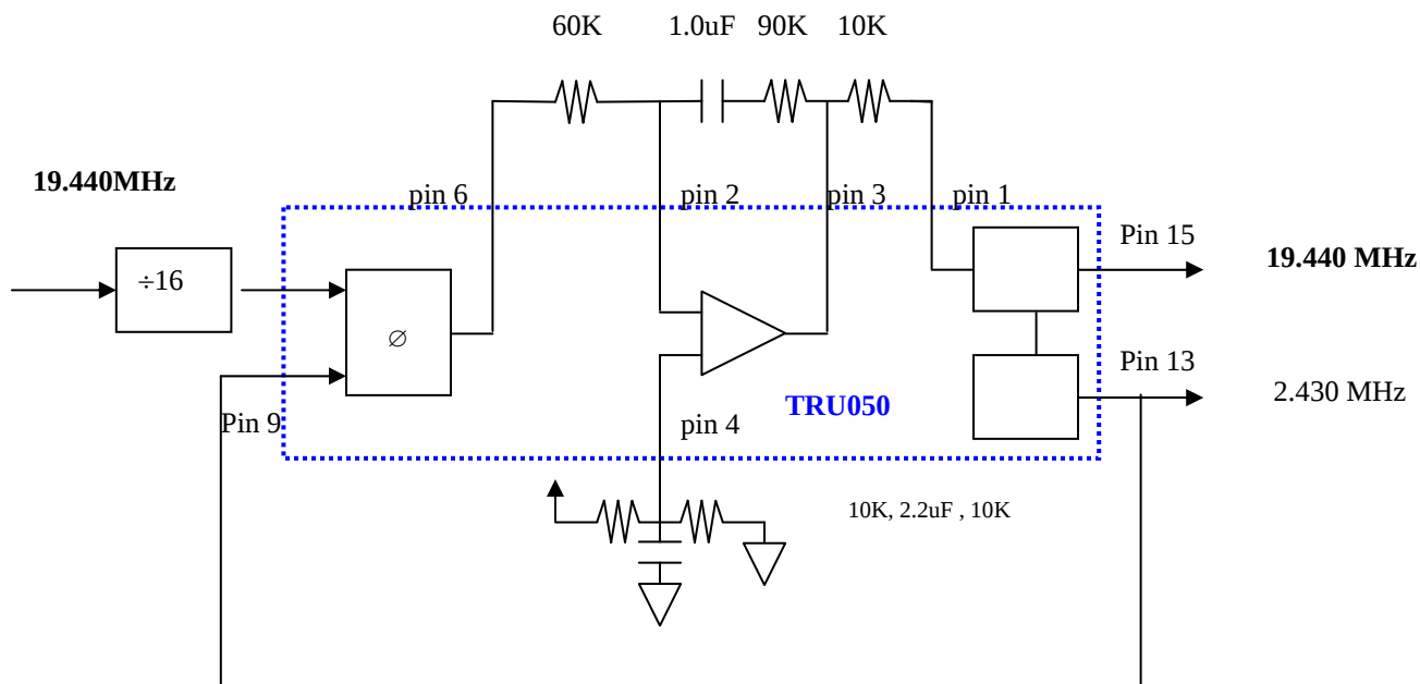
Figure 11. 19.440 Clock Smoothing
