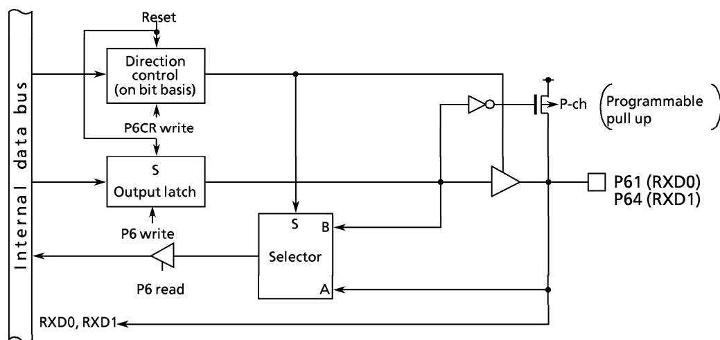
Figure 3.5.11 Ports 61 and 64
