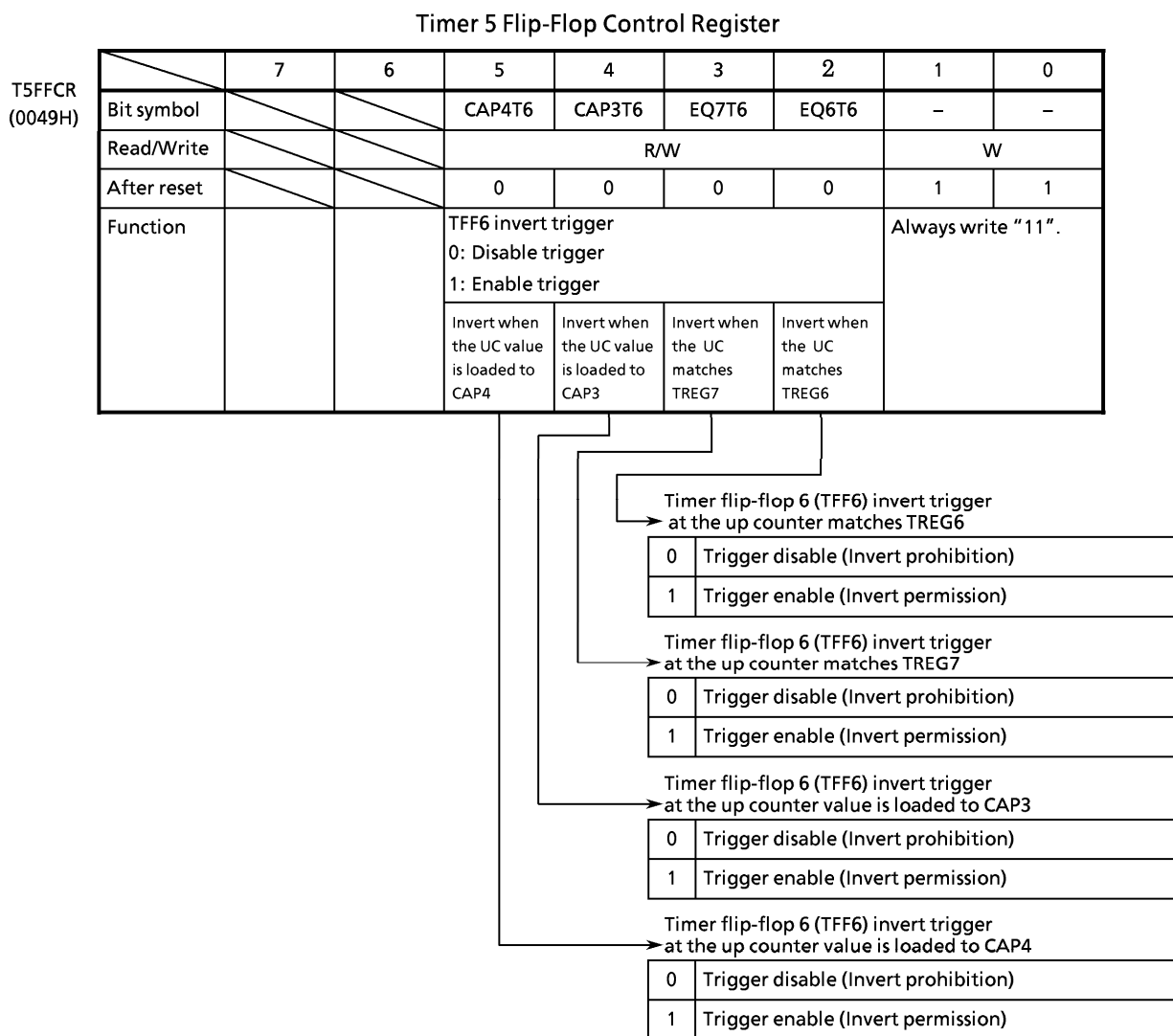
Figure 3.7.6 16-Bit Timer/Event Counter Related Register (4/6)
