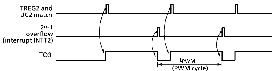
Figure 3.6.16 8-Bit PWM Waveforms
