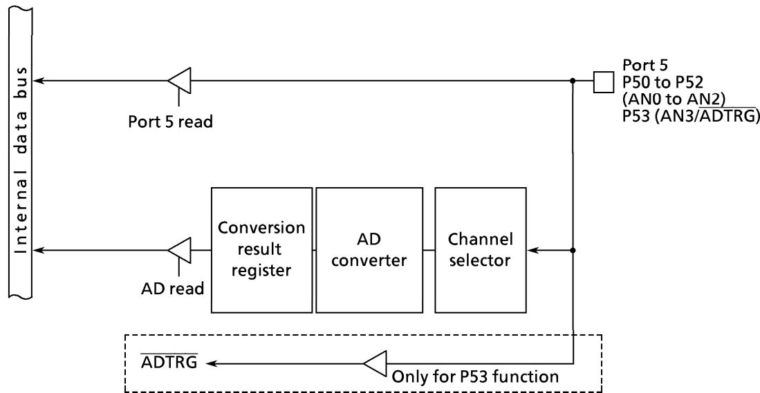
Figure 3.5.8 Port 5
