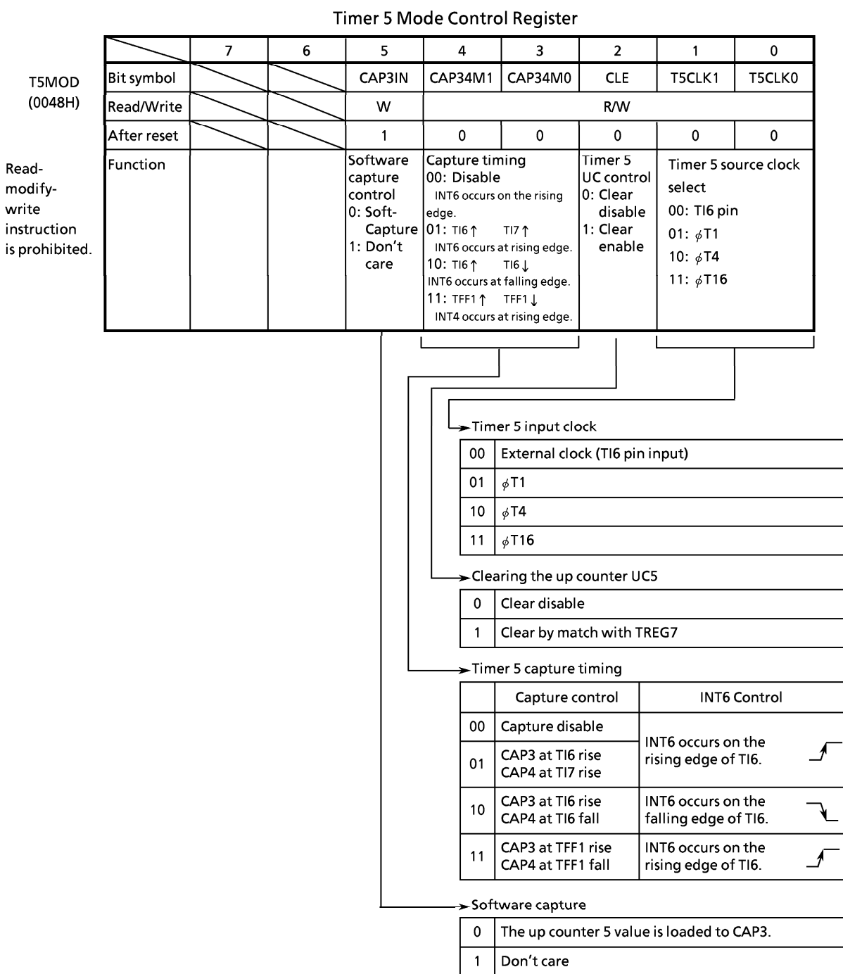
Figure 3.7.5 16-Bit Timer/Event Counter Related Register (3/6)
