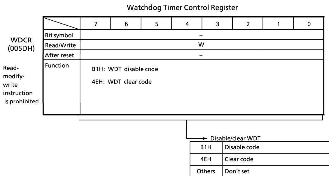
Figure 3.10.4 Watchdog Timer Related Register (2/2)
