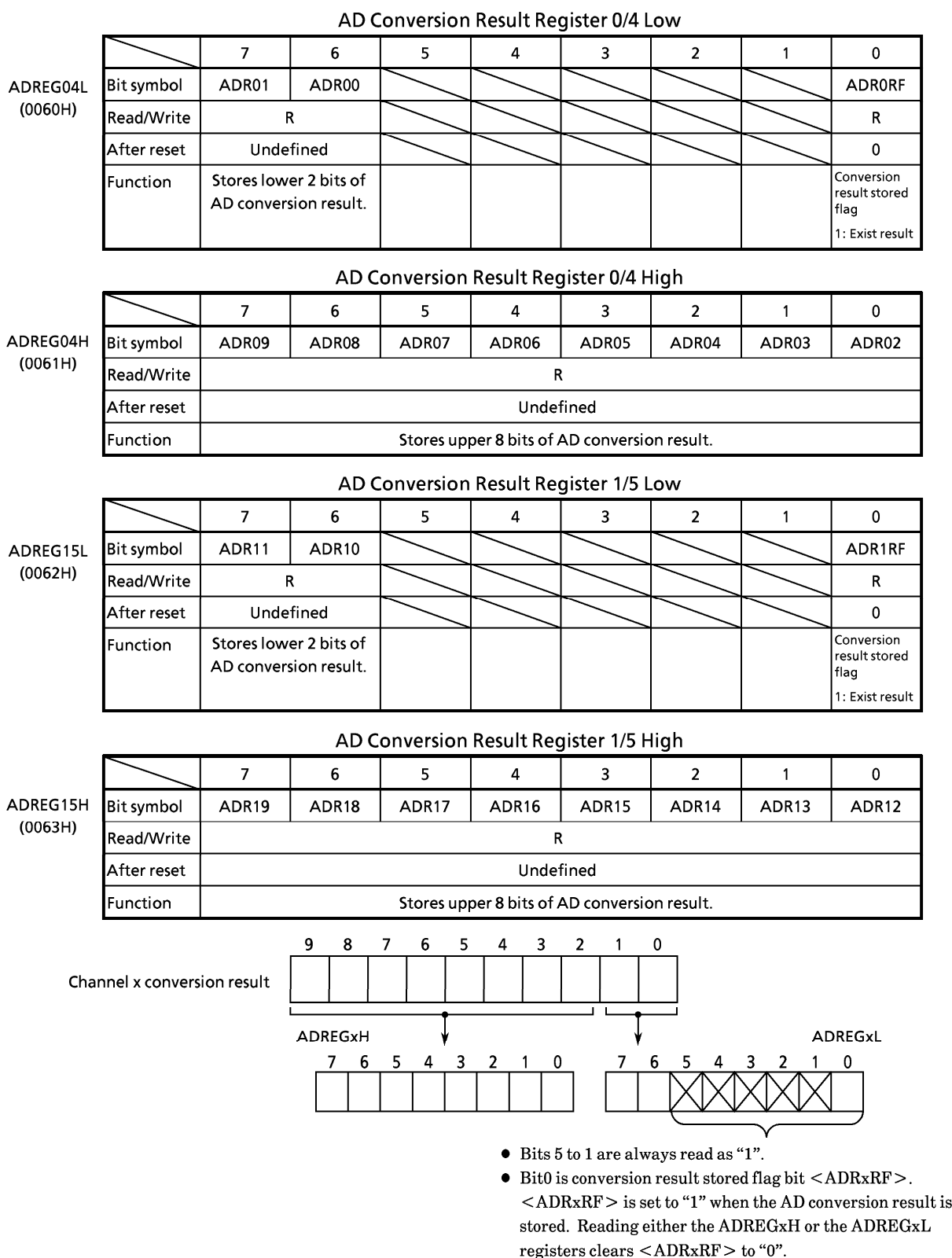
Figure 3.9.4 Registers for AD Converter (3/4)
