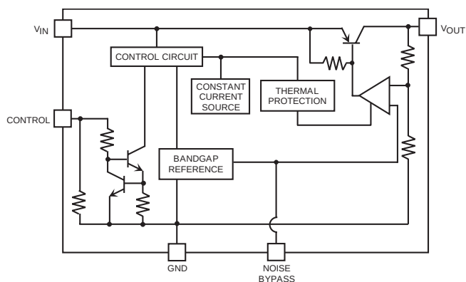
BLOCK DIAGRAM
