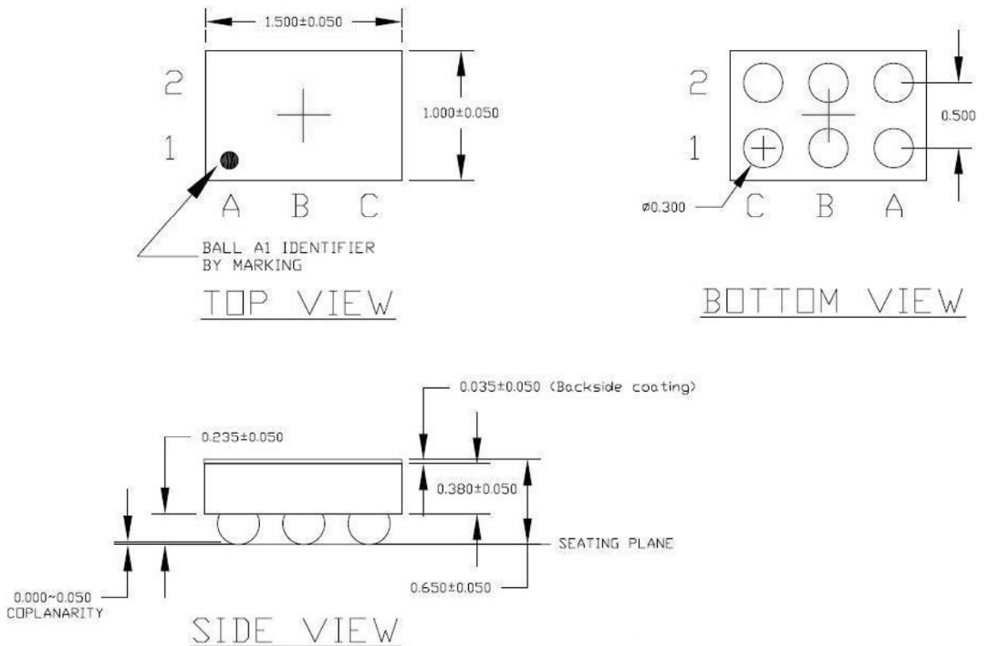
6-Bump, 0.5mm Pitch 1.5mm x 1.0mm Wafer Level Chip-Scale Package (CS)
