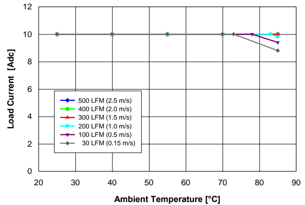
Fig. 3.3V.2: Available load current vs. ambient temperature and airflow rates for YNV12T10033 converter mounted horizontally with V_{in} = 12V , and maximum MOSFET temperature \leq 120^\circ C .
