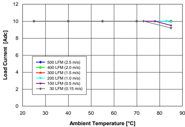
Fig. 3.3V.1: Available load current vs. ambient temperature and airflow rates for YNV12T10033 converter mounted vertically with V_{in} = 12V , and maximum MOSFET temperature \leq 120^\circ C .
