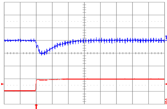
Fig. 1.8V.7: Output voltage response (YNV12T10018) to positive load current step change from 5 \text{ A} to 10 \text{ A} with slew rate of 5 \text{ A}/\mu\text{s} at V_{in} = 12 \text{ V} . Top trace: output voltage ( 100 \text{ mV/div.} ); Bottom trace: load current ( 5 \text{ A/div.} ). C_o = 100 \mu\text{F} ceramic. Time scale: 20 \mu\text{s/div.}
