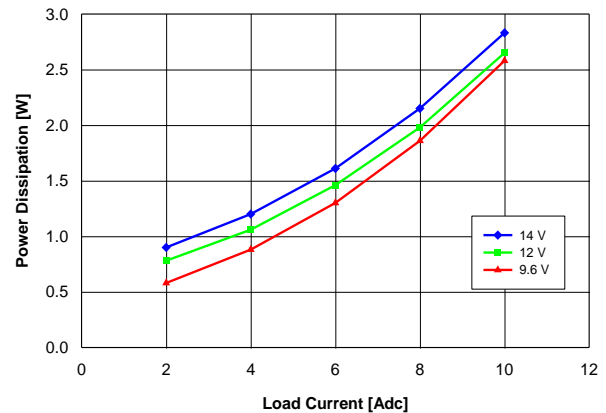
Fig. 3.3V.4: Power loss vs. load current and input voltage for YNV12T10033 converter mounted vertically with air flowing at a rate of 200 LFM (1 m/s) and T_a = 25^\circ C .
