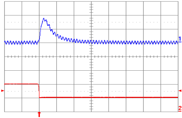
Fig. 5.0V.8: Output voltage response (YNV12T10050) to negative load current step change from 10 A to 5 A with slew rate of -5 A/μs at V_{in} = 12V . Top trace: output voltage (100 mV/div.); Bottom trace: load current (5 A/div.). C_o = 100 \mu F ceramic. Time scale: 20 μs/div.
