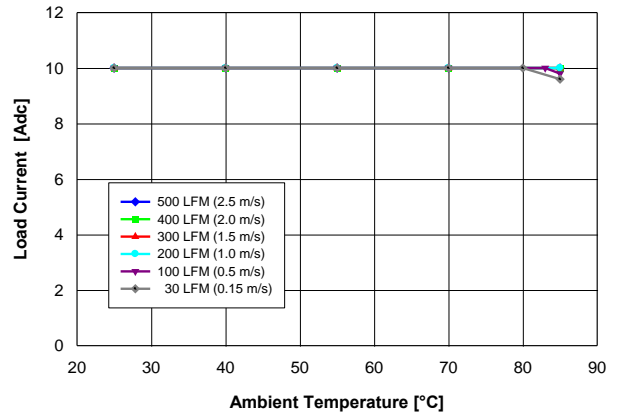
Fig. 1.8V.2: Available load current vs. ambient temperature and airflow rates for YNV12T10018 converter mounted horizontally with Vin = 12 V, and maximum MOSFET temperature ≤ 120 °C.
