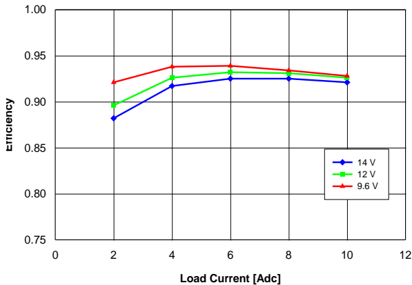
Fig. 3.3V.3: Efficiency vs. load current and input voltage for YNV12T10033 converter mounted vertically with air flowing at a rate of 200 LFM (1 m/s) and T_a = 25^\circ C .
