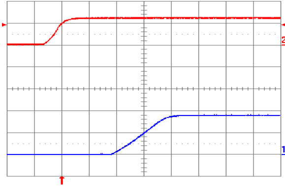
Fig. 1.8V.5: Turn-on transient (YNV12T10018) with application of V_{in} at full rated load current (resistive) and 100 \mu\text{F} external capacitance at V_{in} = 12 \text{ V} . Top trace: V_{in} ( 10 \text{ V/div.} ); Bottom trace: output voltage ( 1 \text{ V/div.} ); Time scale: 2 \text{ ms/div.}
