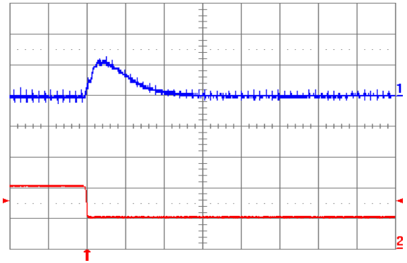
Fig. 1.2V.8: Output voltage response (YNV12T10012) to negative load current step change from 10 A to 5 A with slew rate of -5 A/μs at Vin = 12 V. Top trace: output voltage (100 mV/div.); Bottom trace: load current (5 A/div.). Co = 100 μF ceramic. Time scale: 20 μs/div.
