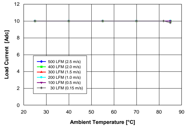
Fig. 1.5V.2: Available load current vs. ambient temperature and airflow rates for YNV12T10015 converter mounted horizontally with V_{in} = 12 \text{ V} , and maximum MOSFET temperature \leq 120 \text{ }^\circ\text{C} .
