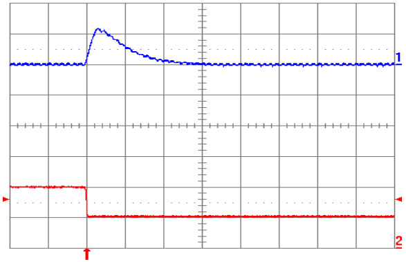
Fig. 2.0V.8: Output voltage response (YNV12T10020) to negative load current step change from 10 A to 5 A with slew rate of -5 A/μs at Vin = 12 V. Top trace: output voltage (100 mV/div.); Bottom trace: load current (5 A/div.). Co = 100 μF ceramic. Time scale: 20 μs/div.
