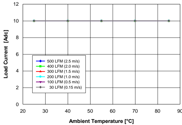
Fig. 1.5V.1: Available load current vs. ambient temperature and airflow rates for YNV12T10015 converter mounted vertically with V_{in} = 12 \text{ V} , and maximum MOSFET temperature \leq 120 \text{ }^\circ\text{C} .
