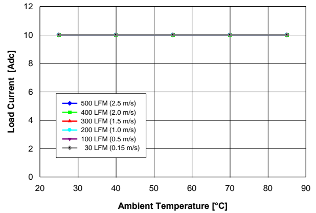
Fig. 1.0V.2: Available load current vs. ambient temperature and airflow rates for YNV12T10010 converter mounted horizontally with Vin = 12 V, and maximum MOSFET temperature ≤ 120 °C.
