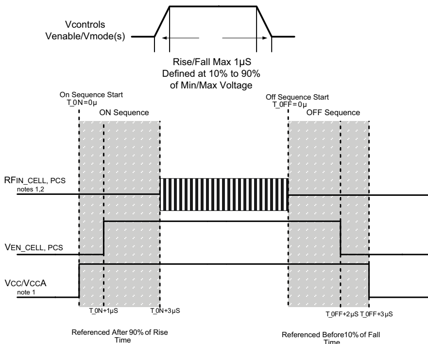
Figure 3: Recommended ON/OFF Timing Sequence
