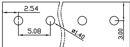
PCB Layout
