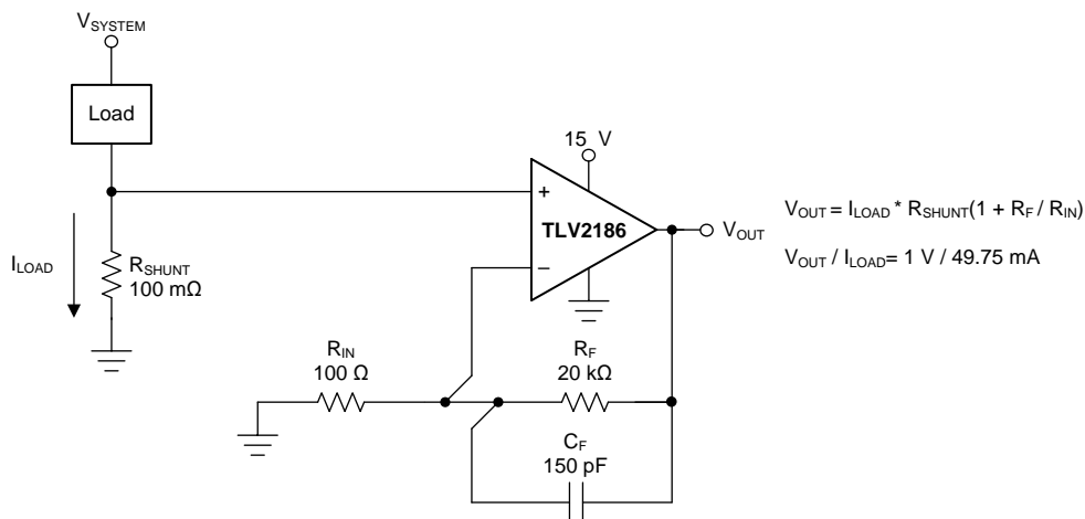
Figure 49. Low-Side Current Monitor
