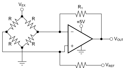
Figure 48. Bridge Amplifier
