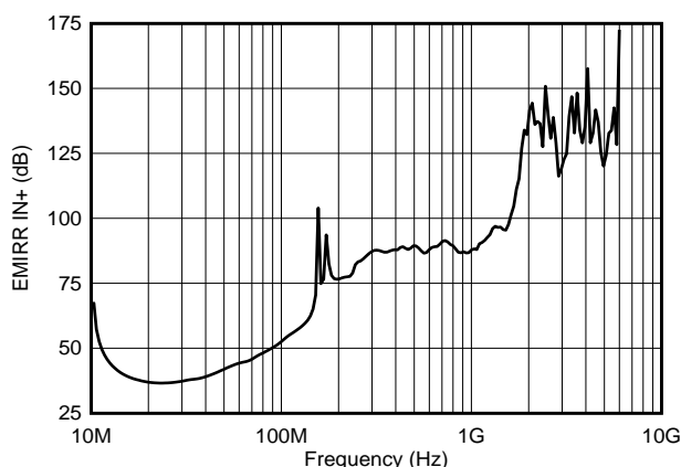
Figure 40. EMIRR Testing
