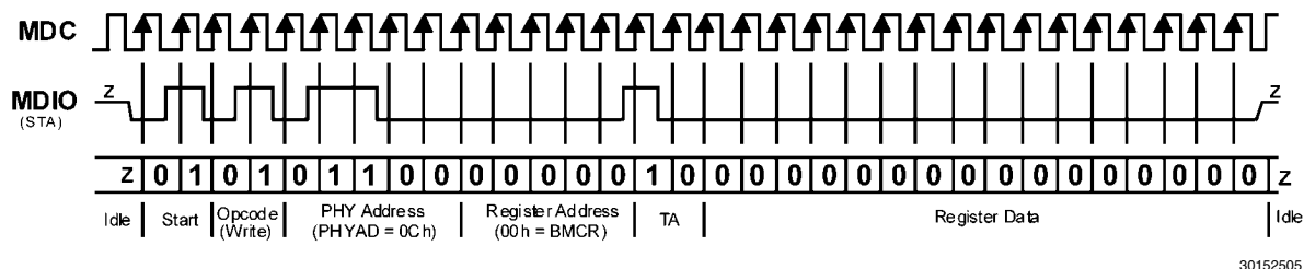
FIGURE 4. Typical MDC/MDIO Write Operation
