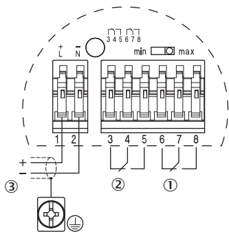
Double relay connection diagram
