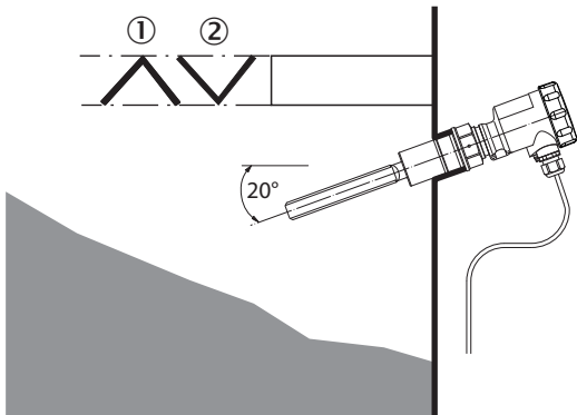
Horizontal mounting
