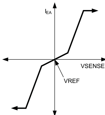
Figure 28. Basic Voltage-Error Amplifier Transconductance Curve
