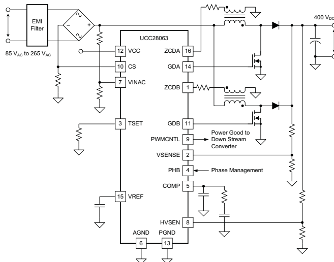
Typical Application Diagram
