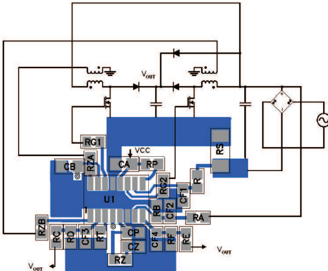
Figure 35. Recommended PCB Layout
