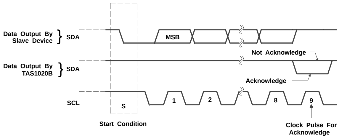
Figure 2–13. TAS1020B Acknowledge on the I²C Bus
