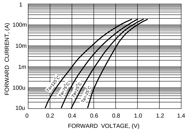
FIG. 2 - FORWARD CHARACTERISTICS
