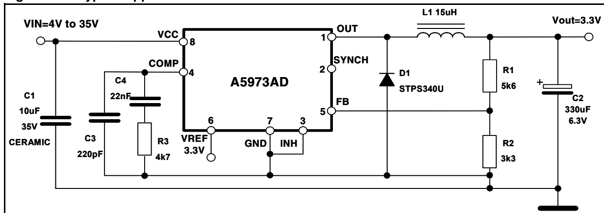
Figure 1. Typical application
