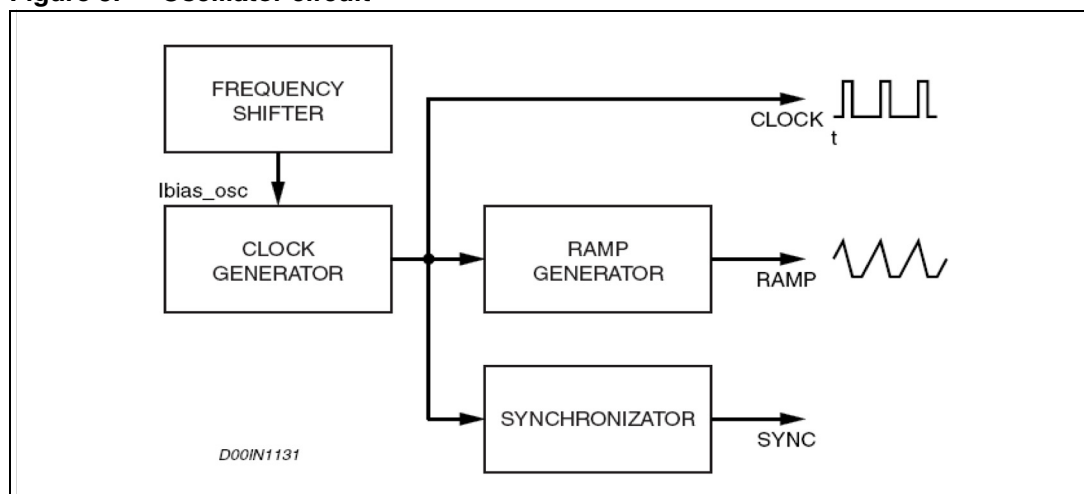
Figure 5. Oscillator circuit
