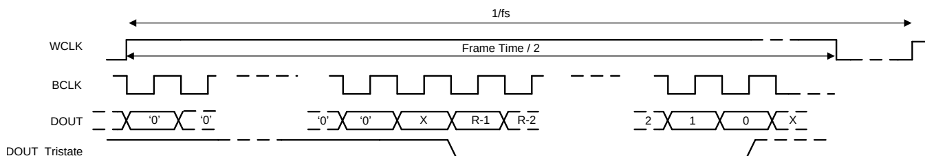
Figure 11. First Channel Disabled, Second Channel Enabled, Tri-Stating Enabled
