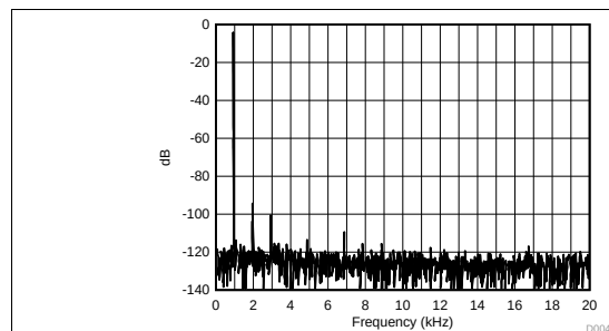
Figure 139. Line Input to ADC FFT Plot
