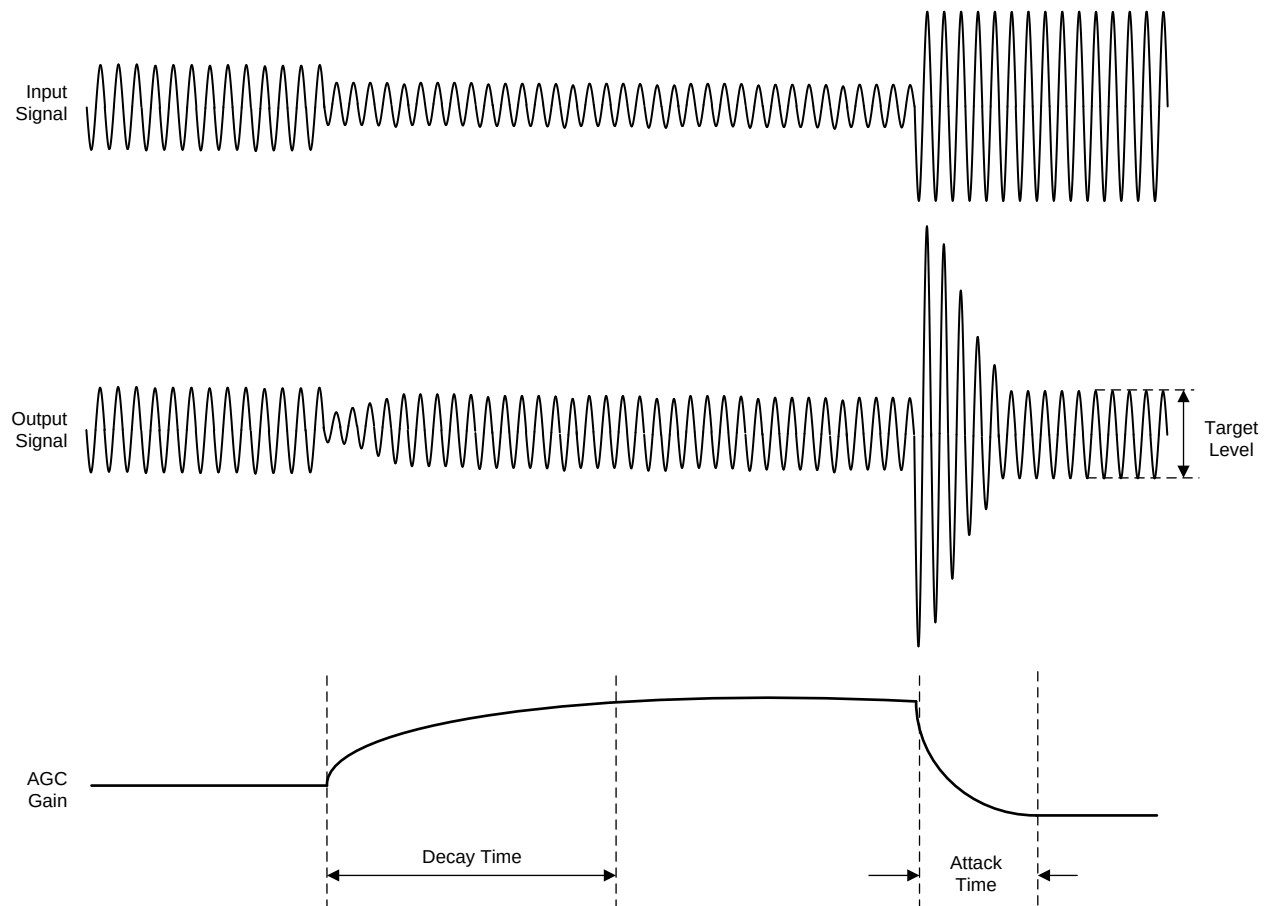
Figure 28. AGC Characteristics
