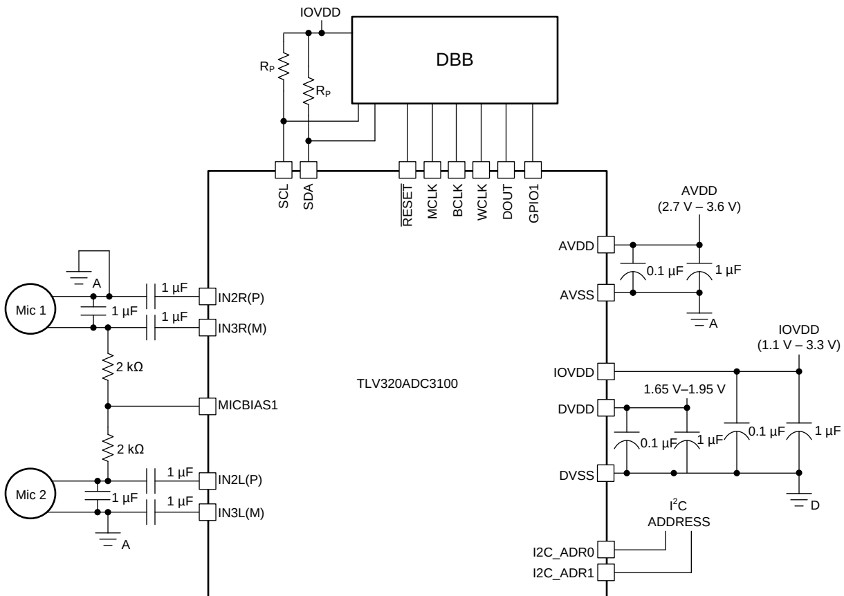
Figure 137. Typical Connections
