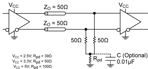
Figure 3. Three Resistor "Y Termination"
