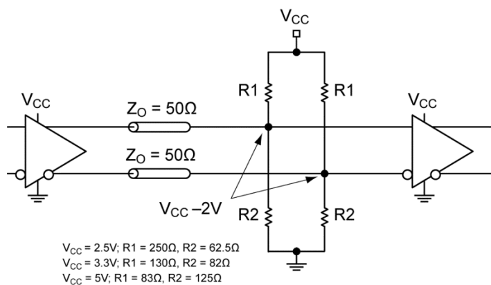
Figure 2. Parallel Thevenin-Equivalent Termination
