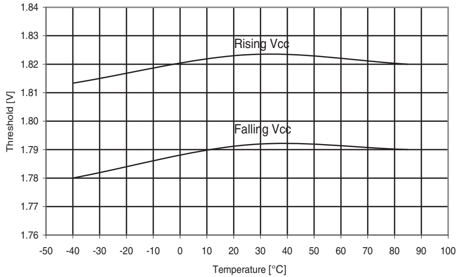
Figure 30-229. ATmega644A: BOD threshold vs. temperature ( V_{BOT} = 1.8V )
