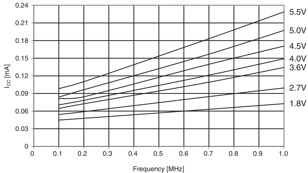
Figure 30-300. ATmega1284: Idle supply current vs. low frequency (0.1 - 1.0MHz)
