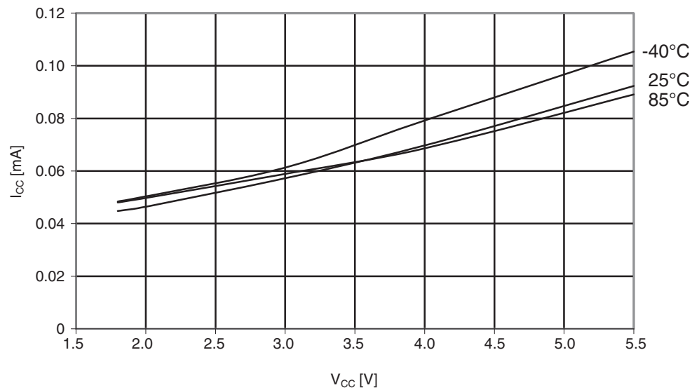
Figure 30-59. ATmega164PA: Idle supply current vs. V_{CC} (internal RC oscillator, 128kHz)
