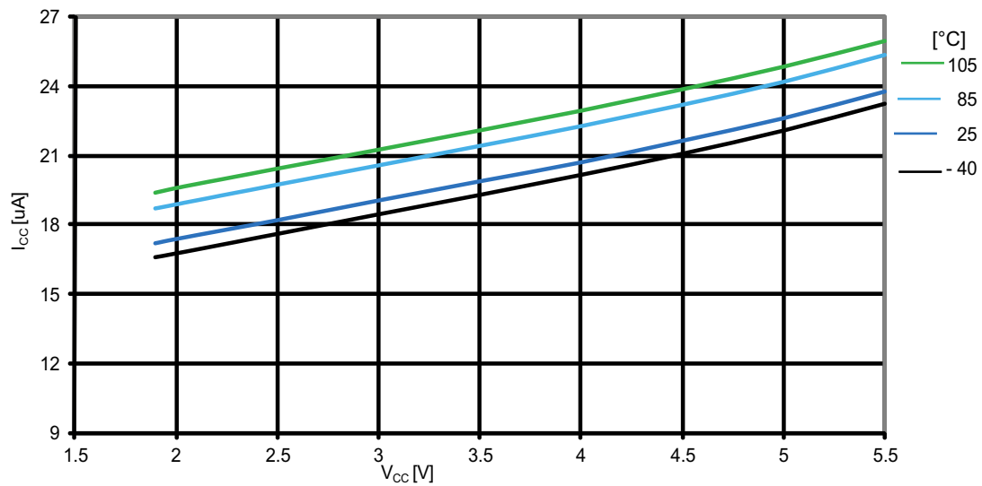
Figure 31-38. ATmega164PA: Brownout detector current vs. V_{CC}
