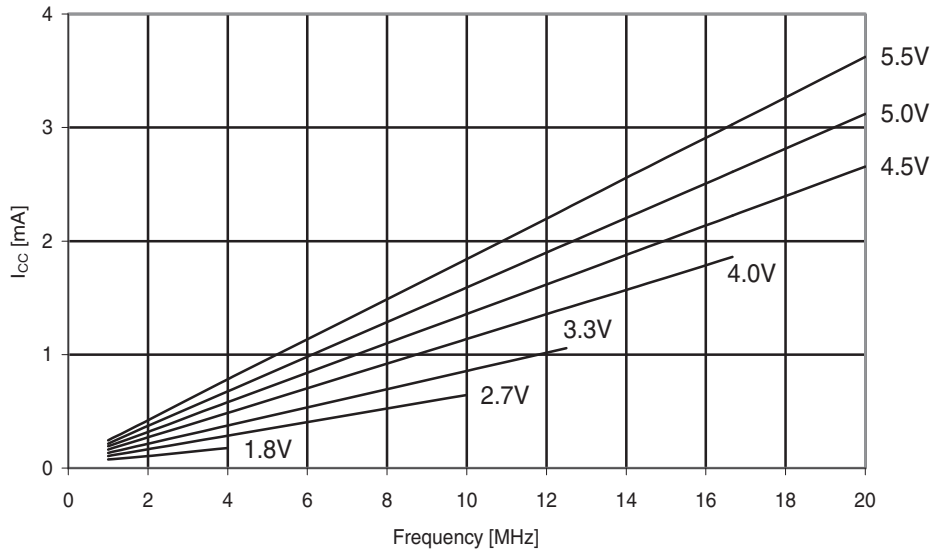
Figure 30-105. ATmega324A: Idle supply current vs. V_{CC} (1 - 20MHz)
