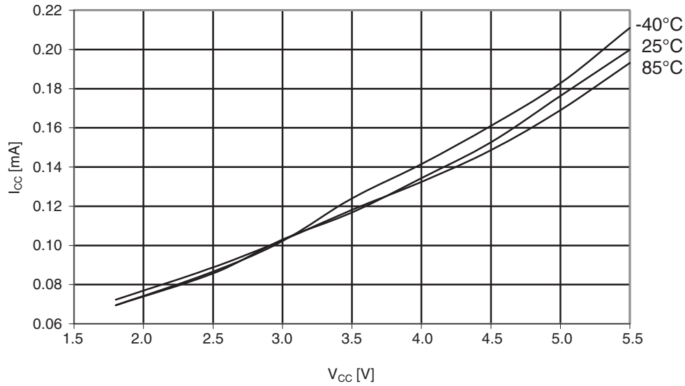
Figure 30-201. ATmega644A: Active supply current vs. V_{CC} (internal RC oscillator, 128kHz)
