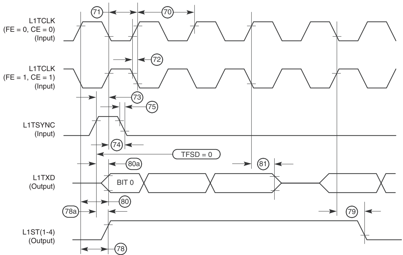
Figure 57. SI Transmit Timing Diagram (DSC = 0)
