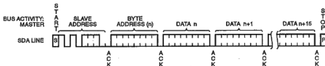
Figure 7. Page Write Timing
