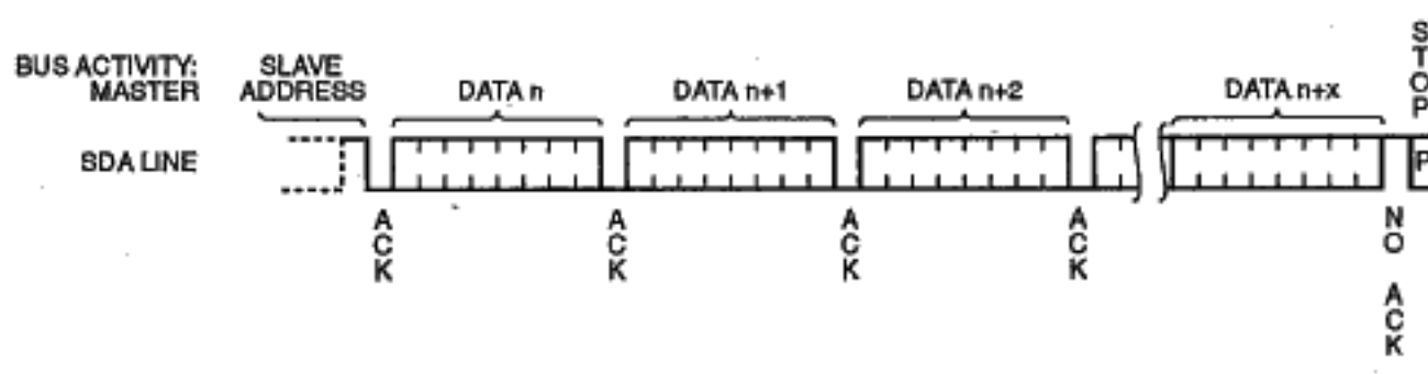
Figure 10. Sequential Read Timing
