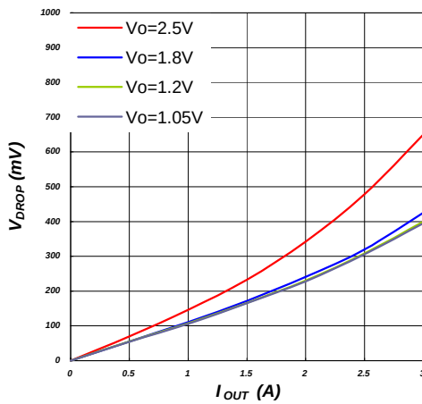
Dropout Voltage at V_{CTL} = 5V
