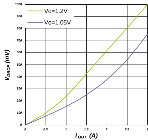
Dropout Voltage at V_{CTL} = 3.3V
