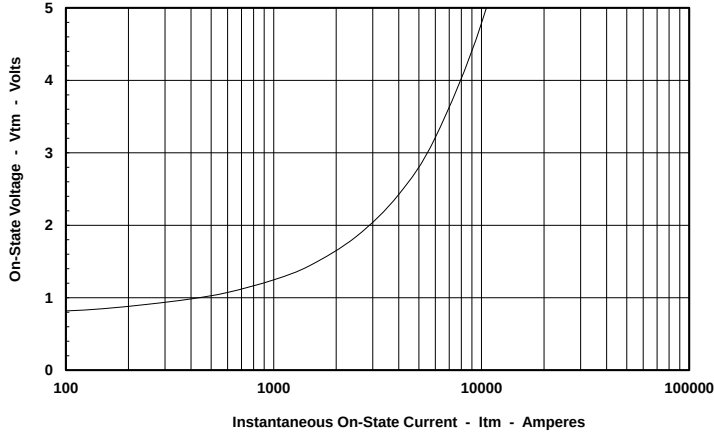
Maximum On-State Forward Voltage Drop ( T_J = 130^\circ\text{C} )
