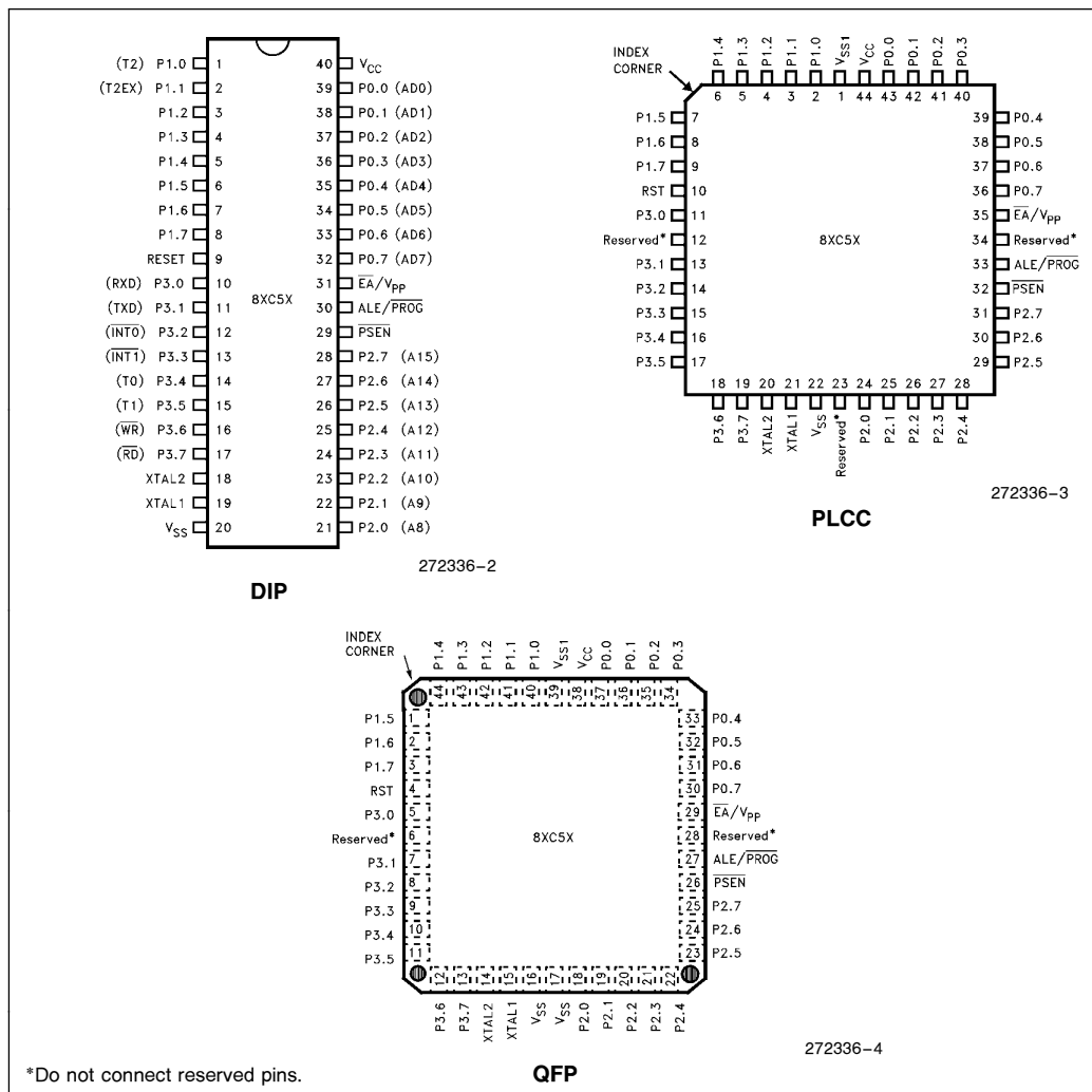
Figure 2. Pin Connections
