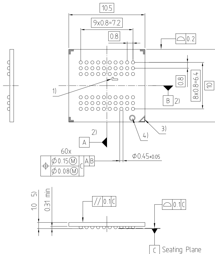
FIGURE 5 60-ball PG-VFBGA-60-4 (x16)
