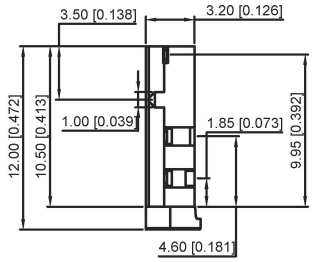
(Ø3.50mm 4 POLE PLUG DETAIL DRAWING)
