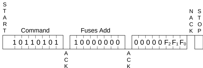
Figure 7. Read Fuses
