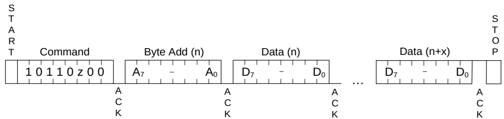
Figure 6. Write Zone
