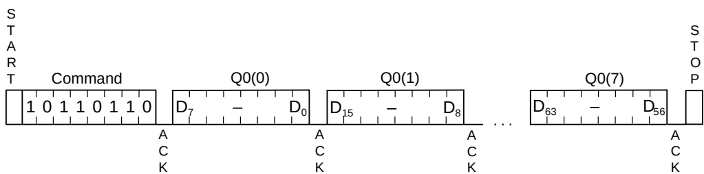
Figure 11. Initialize Authentication
