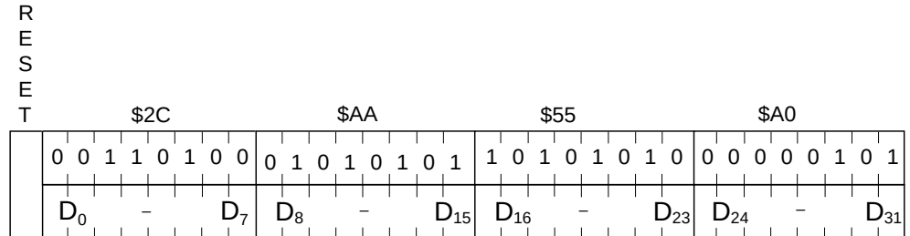
Figure 9. Answer-to-reset
