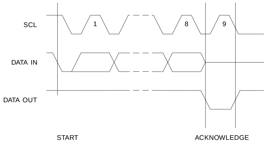
Figure 15. Output Acknowledge
