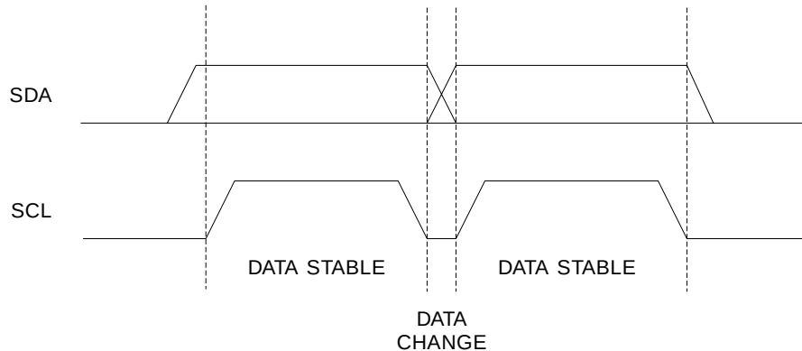
Figure 14. Data Validity
