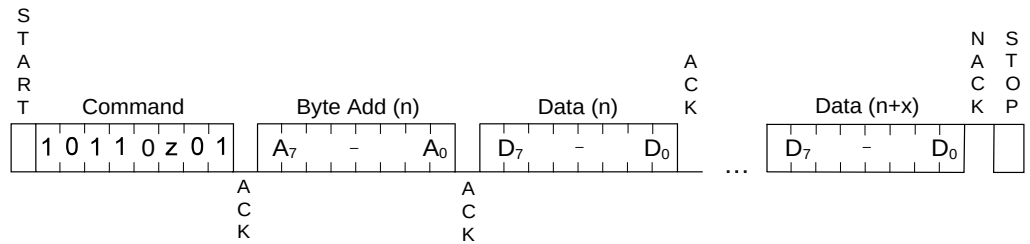
Figure 5. Read Zone
