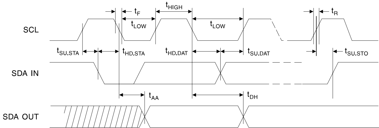
Figure 16. Bus Timing
