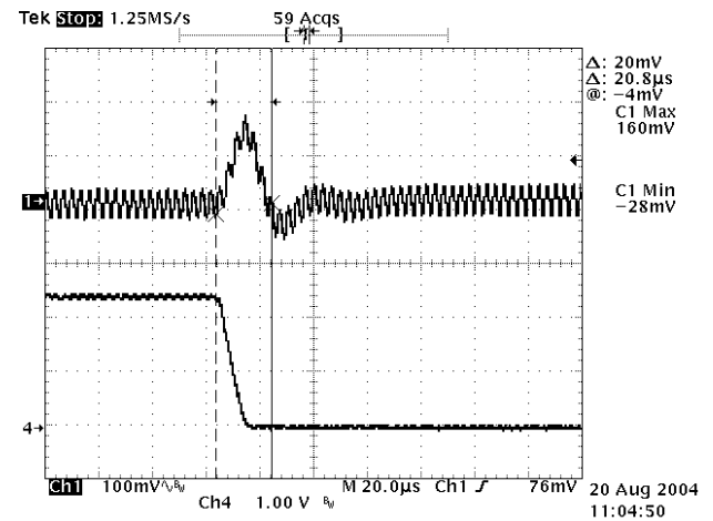
Figure 22: Typical transient response to step load change at 0.5A/μS from 50% to 0% of Io, max at 5.0Vin, 2.5V out (measurement with a 1μF ceramic and a 10μF tantalu)
