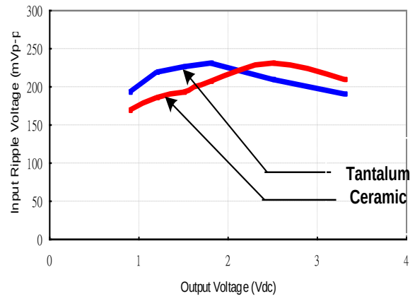
Figure 26: Input ripple voltage for various output models, I_O = 6A ( C_{in} = 2x100\mu F tantalum capacitors or 2x22\mu F ceramic capacitors at the input)
