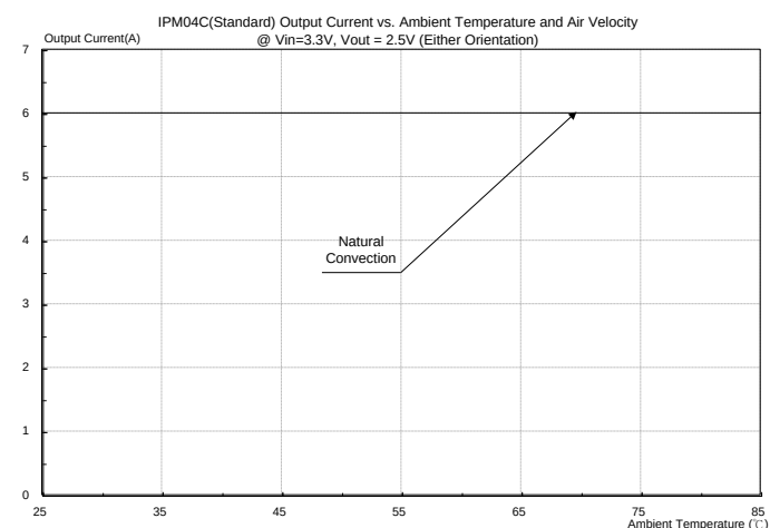
Figure 36: Output current vs. ambient temperature and air velocity @ Vin=3.3V, Vout=2.5V(Eithere Orientation)
