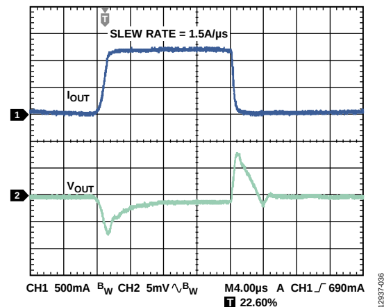
Figure 34. Load Transient Response, I_{\text{LOAD}} = 100\text{mA} to 1.2\text{A} , V_{\text{OUT}} = 3.3\text{V} , V_{\text{IN}} = 4.0\text{V} , C_{\text{OUT}} = 22\mu\text{F} , Channel 1 = I_{\text{OUT}} , Channel 2 = V_{\text{OUT}}
