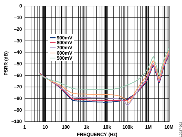
Figure 22. Power Supply Rejection Ratio (PSRR) vs. Frequency at Various Headroom Voltages, V_{OUT} = 3.3\text{ V} , 1.2\text{ A Load}
