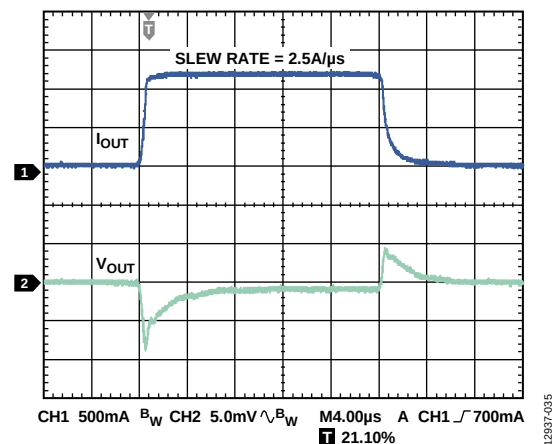
Figure 33. Load Transient Response, I_{\text{LOAD}} = 100\text{mA} to 1.2\text{A} , V_{\text{OUT}} = 3.3\text{V} , V_{\text{IN}} = 4.0\text{V} , Channel 1 = I_{\text{OUT}} , Channel 2 = V_{\text{OUT}}
