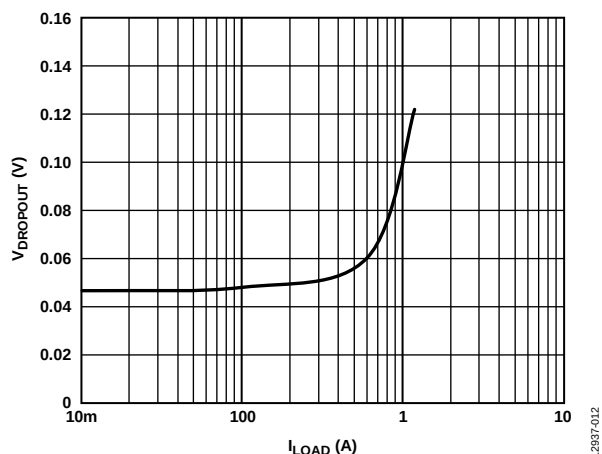
Figure 12. Dropout Voltage ( V_{DROP} ) vs. Load Current ( I_{LOAD} ), V_{OUT} = 3.3\text{ V}
