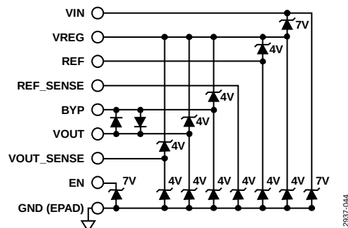
Figure 42. Simplified ESD Protection Block Diagram
