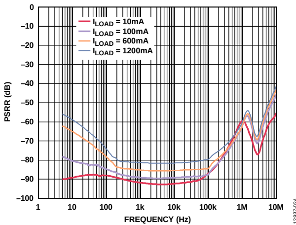
Figure 24. Power Supply Rejection Ratio (PSRR) vs. Frequency at Various Loads, V_{OUT} = 1.8\text{ V} , V_{IN} = 2.6\text{ V}
