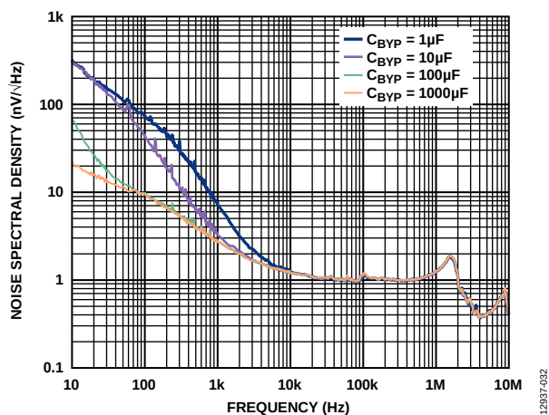
Figure 30. Noise Spectral Density vs. Frequency at Various Values of C_{\text{BYP}}
