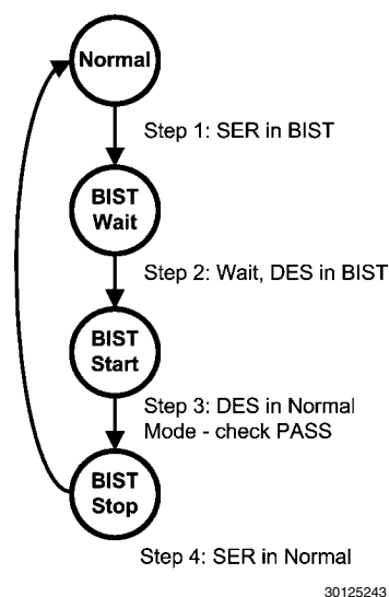
FIGURE 25. BIST Mode Flow Diagram
