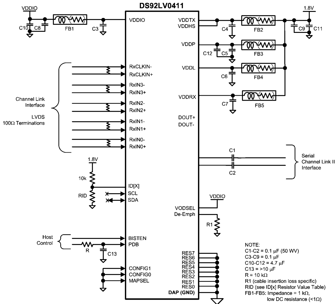
FIGURE 31. DS92LV0411 Typical Connection Diagram
