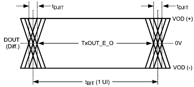
FIGURE 12. Output Jitter
