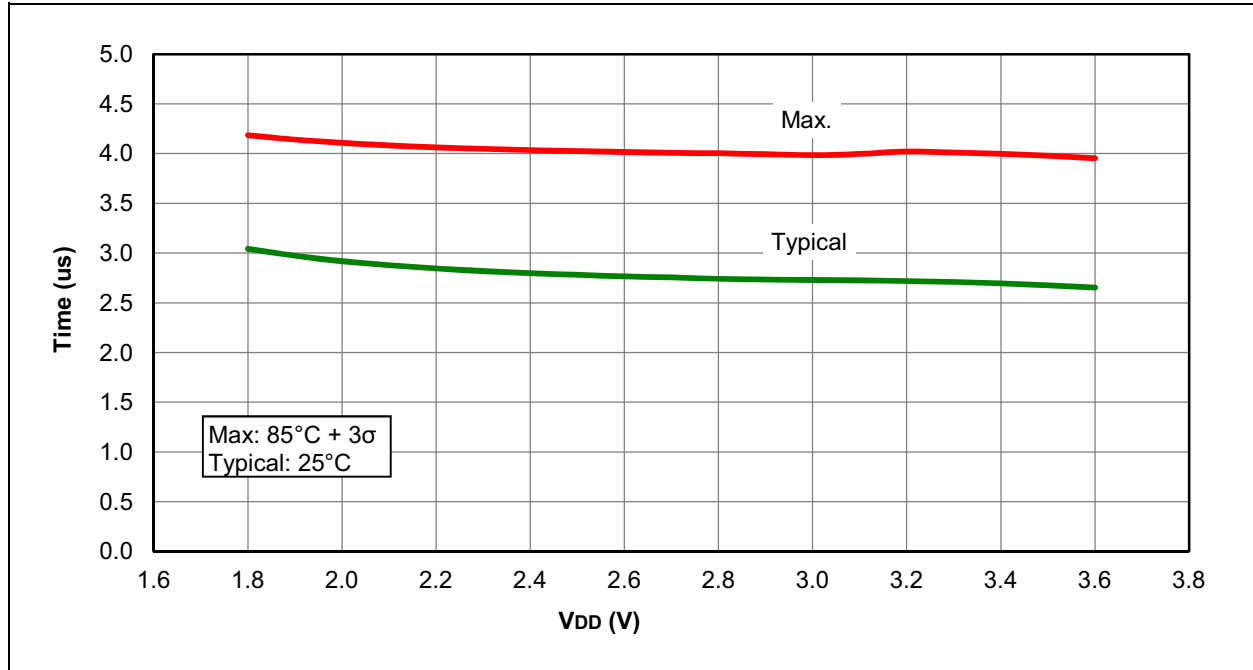
FIGURE 26-53: SLEEP MODE, WAKE PERIOD WITH HFINTOSC SOURCE, PIC16LF1507 ONLY
