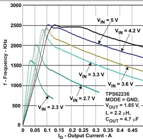
Figure 25. Switching Frequency vs Output Current, 1.85-V Output Voltage, PFM/PWM Mode – TPS62236
