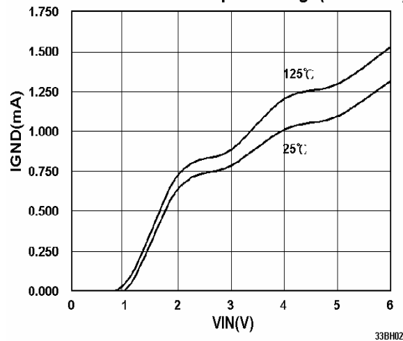
Ground Pin Current Vs Input Voltage (V SD =V IN )
