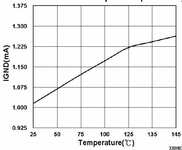
Ground Current Vs Temperature (V SD =V IN )
