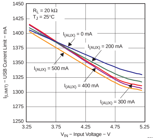
Figure 17. USB Current-Limit Threshold vs V_{IN} , R_{LIM} = 20\text{ k}\Omega , T_A = 25^\circ\text{C}
