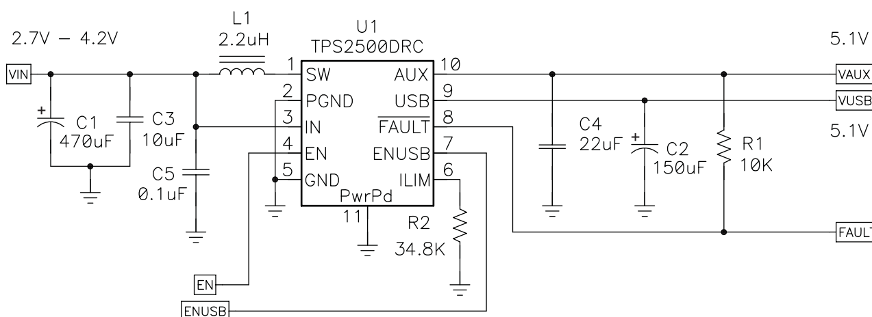
Figure 22. Reference Schematic
