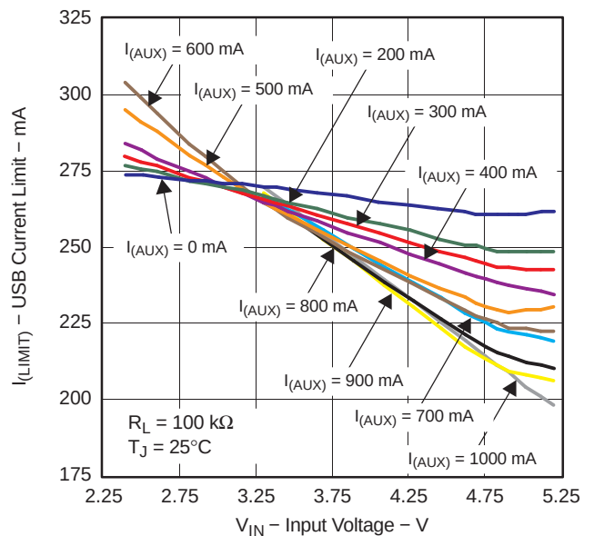
Figure 19. USB Current-Limit Threshold vs V_{IN} , R_{LIM} = 100\text{ k}\Omega , T_A = 25^\circ\text{C}
