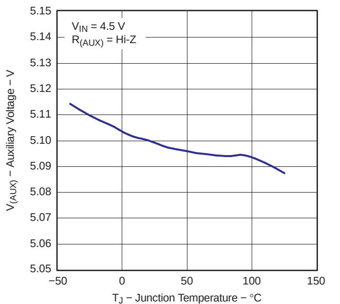
Figure 6. V_{AUX} vs Junction Temperature, I_{AUX} = I_{USB} = 0 A
