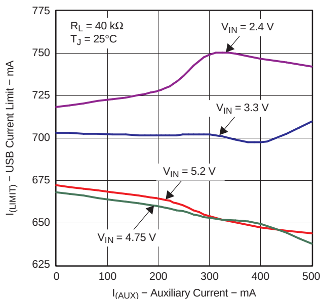
Figure 15. USB Current-Limit Threshold vs I_{AUX} , R_{ILIM} = 40\text{ k}\Omega , T_A = 25^\circ\text{C}
