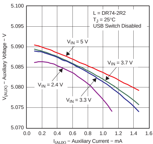
Figure 27. Load Regulation, TPS2501 (Forced PWM Mode)
