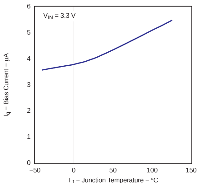
Figure 9. Bias Current vs Junction Temperature, V_{IN} = 3.3\text{ V} , V_{EN} = 0\text{ V} (Disabled)
