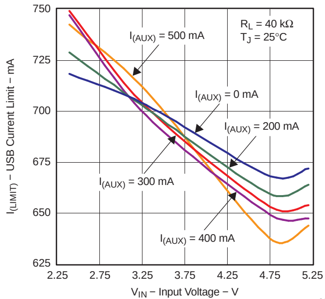
Figure 18. USB Current-Limit Threshold vs V_{IN} , R_{LIM} = 40\text{ k}\Omega , T_A = 25^\circ\text{C}
