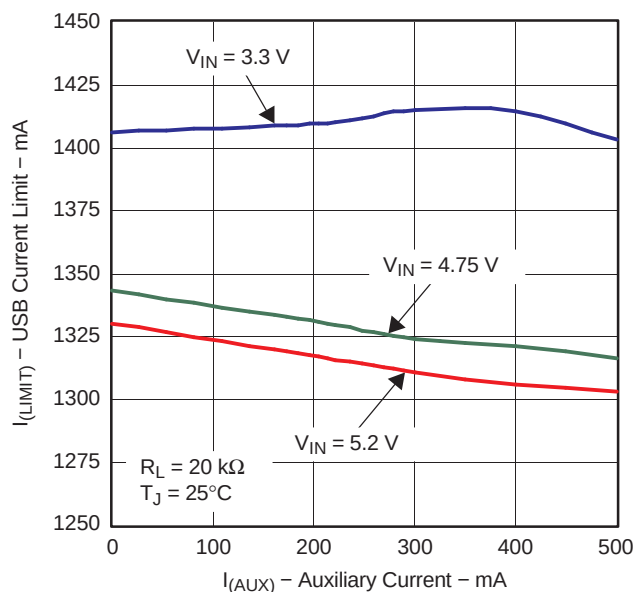
Figure 14. USB Current-Limit Threshold vs I_{AUX} , R_{ILIM} = 20\text{ k}\Omega , T_A = 25^\circ\text{C}
