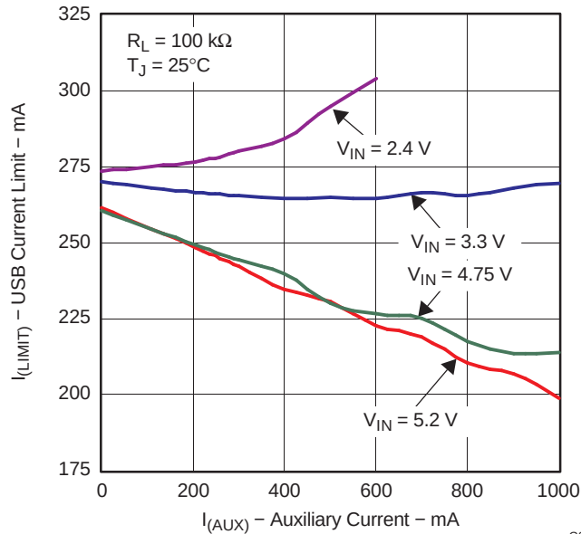
Figure 16. USB Current-Limit Threshold vs I_{AUX} , R_{LIM} = 100\text{ k}\Omega , T_A = 25^\circ\text{C}
