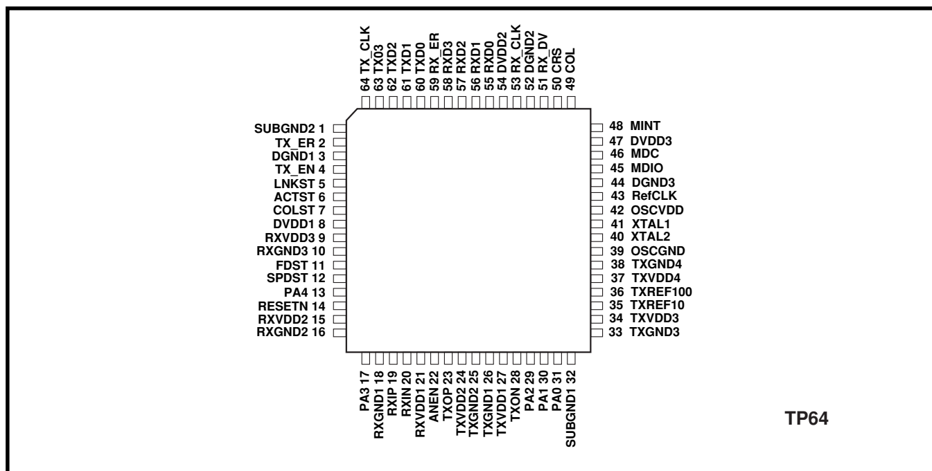
Figure 2Pin connections
