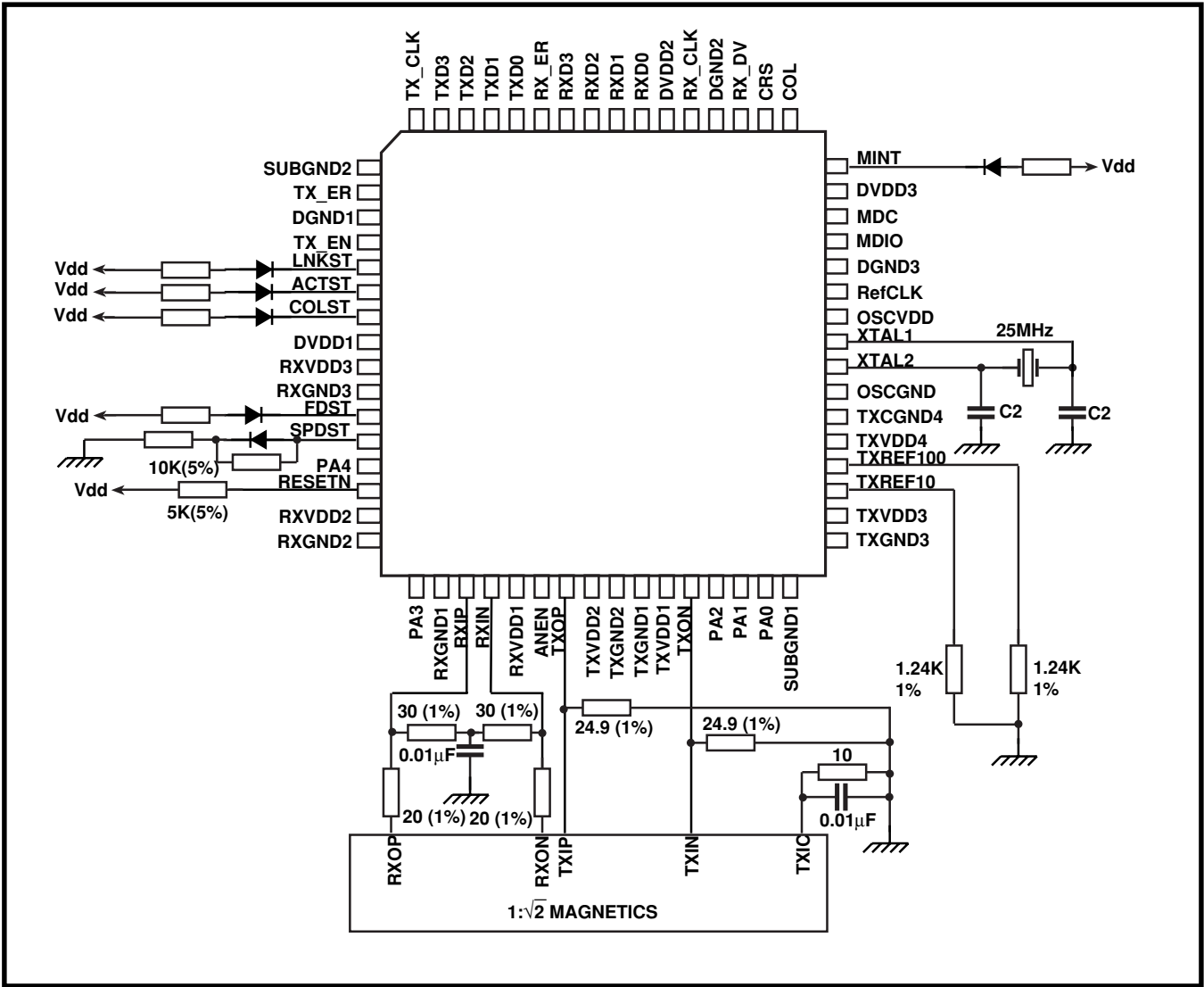
Figure 7 External Components
