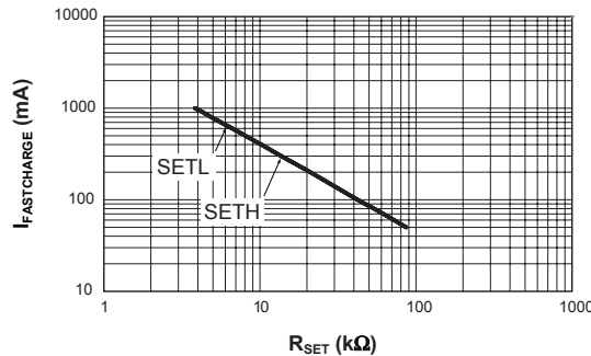
Figure 3: I_{\text{FASTCHARGE}} vs. R_{\text{SET}}
