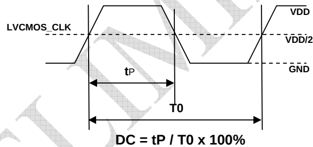
Figure 3. Output Duty Cycle (DC)
