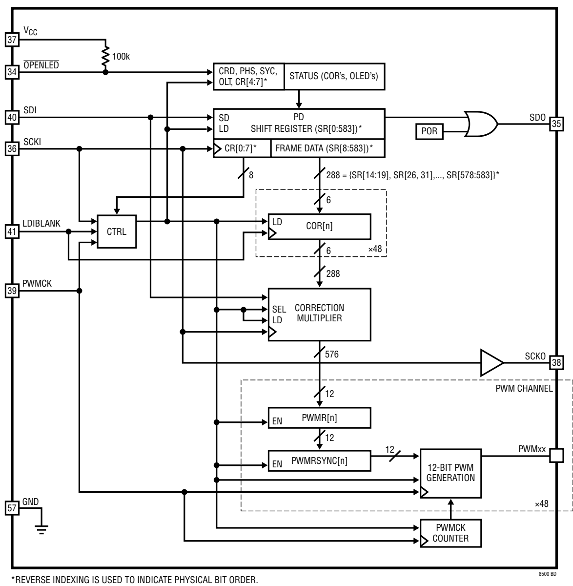
Figure 1. Block Diagram
